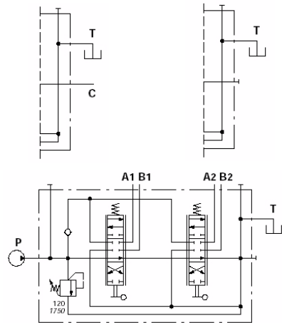
Power beyond
