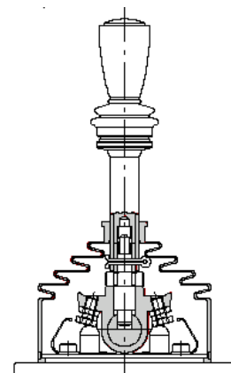
11 Control - Detent in positions 1 and 2. Detent in neutral, lift to release.
