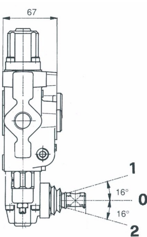
Power beyond
