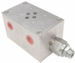
SMC3P1A-R-TT10-30 Tank top c/w relief Nom. flow = 30L/min
