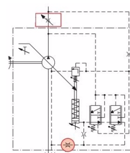
RN0 Torque Control
