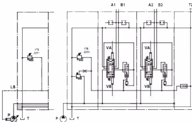
Closed Centre
