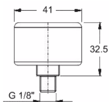
Gauge Horizontal
