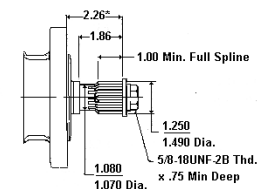
14 Tooth Spline (Code 05)
