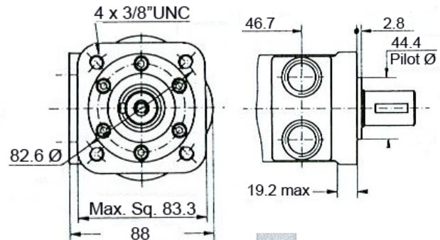
Q Mount
