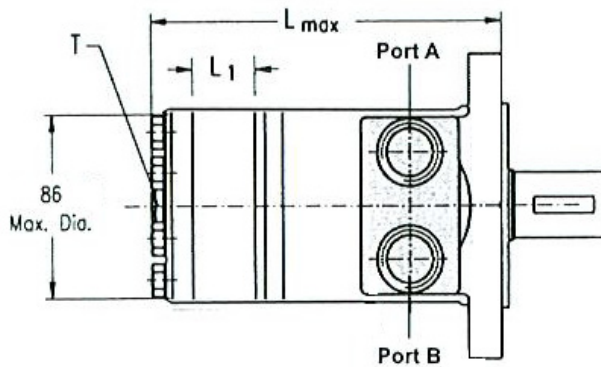
A Mount
