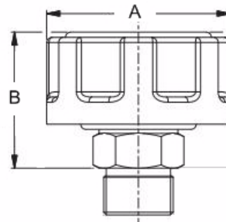
Threaded Filler Breather
