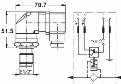
Electrical c/w Thermostat Visual Indicator
