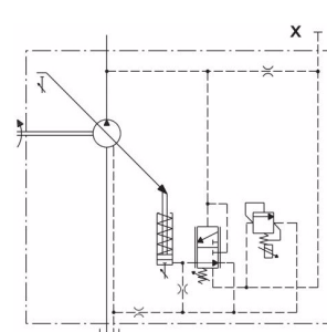
PEC Electro-Prop. Press.Comp.
