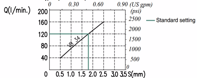
Typical pressure drop vs. flow characteristic
