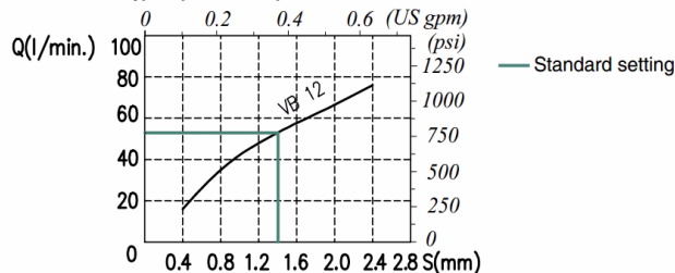
Typical pressure drop vs. flow characteristic
