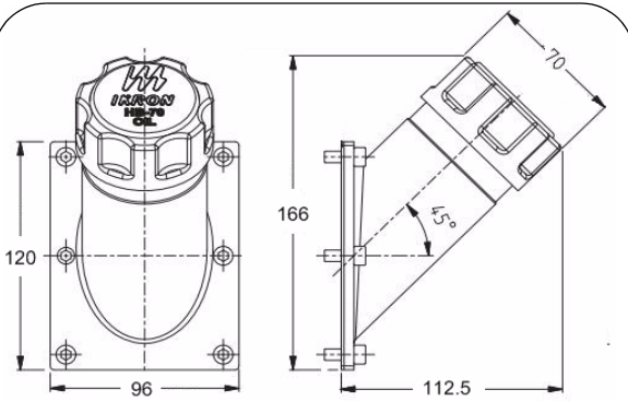
Side Mounted Filler Breather
