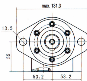
A Mount
