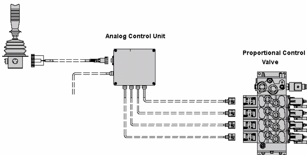
Control joystick
