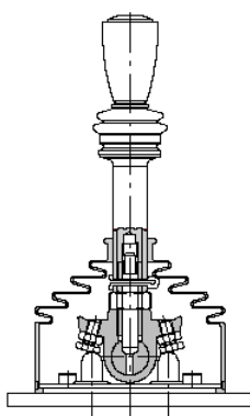
02 Control Detent in neutral, lift to release.
