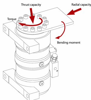
Cantilever Mounting
