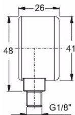
Gauge Vertical
