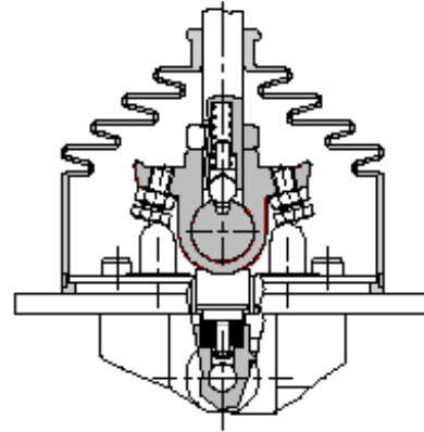
03 Control - With friction (stop in any position) and neutral sensing.
