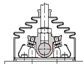
07 Control - Detent in position 1 and 2, spring centred to neutral position.
